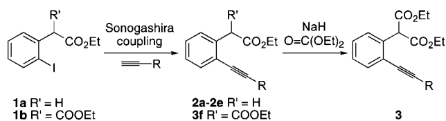
Scheme 1. Synthesis of Alkynyl Malonates 3
