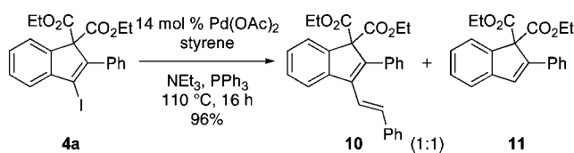
Scheme 4. Heck Reaction Using 4a as Substrate
